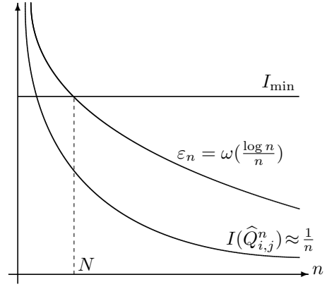
Fig. 1. Graphical interpretation of the condition on \varepsilon_n . As n \rightarrow \infty , the regularization sequence \varepsilon_n will be smaller than I_{\min} and larger than I(\widehat{Q}_{i,j}^n) with high probability.
