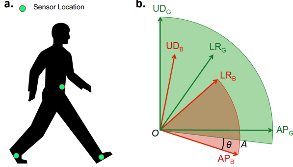
Figure 6. Sensor locations on the body, and the transformation between IMU and Global reference frames.
