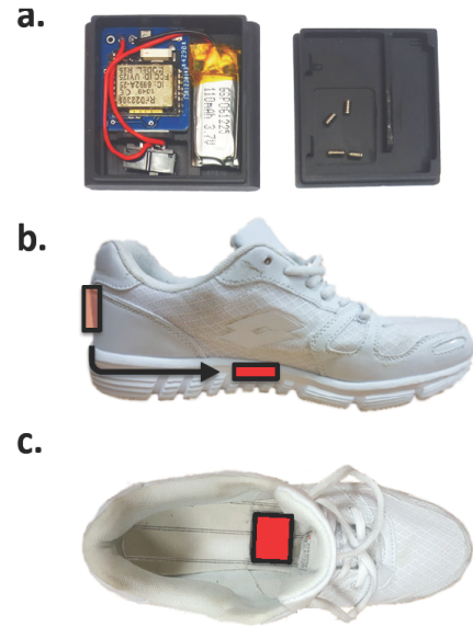
Figure 2. The sensor in its case, and the location of sensor in the shoe.
